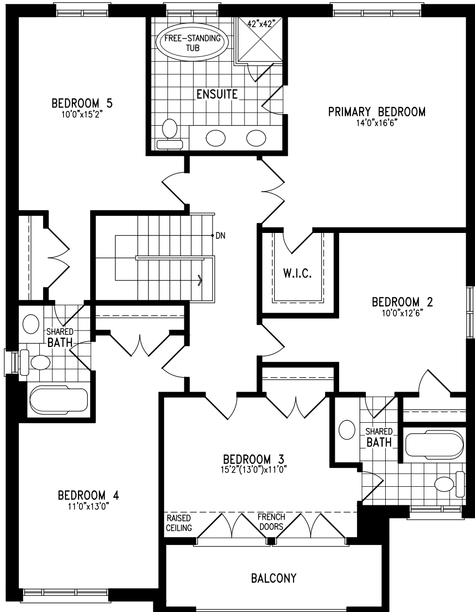
ELEVATION C OPT. SECOND FLOOR W/ 5 BEDROOMS
