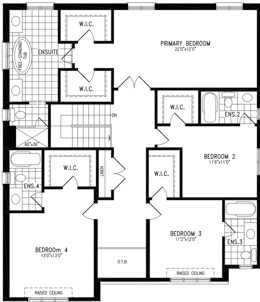
ELEVATION B SECOND FLOOR
